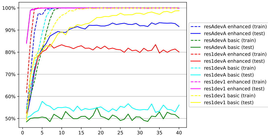
Figure 4: Effect of the number of epochs on the accuracy of classifiers trained with various IoT KGs.
