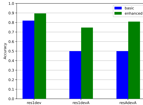
Figure 5: Average accuracies of the classifiers, trained on different amounts of devices, for the full OPSD data.
