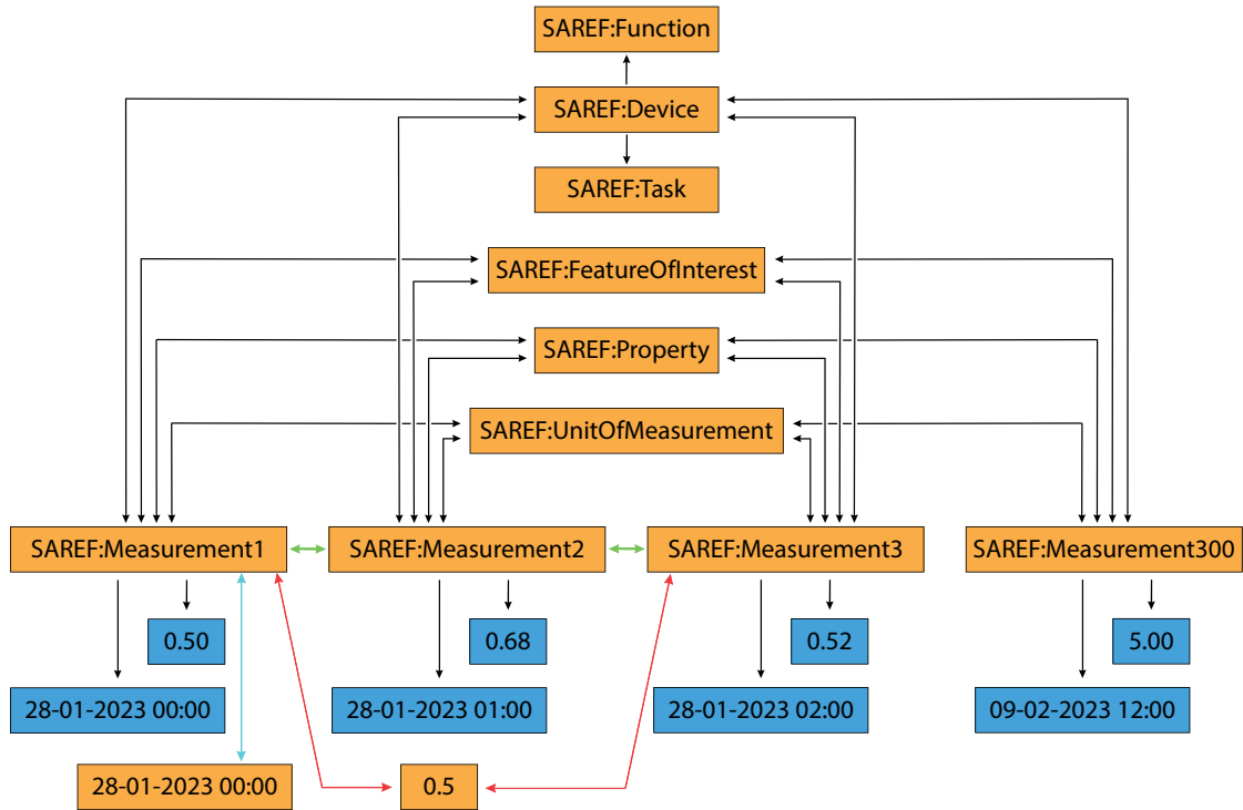
Figure 3: Updated visualization of Figure 1 with the semantic enrichment.
