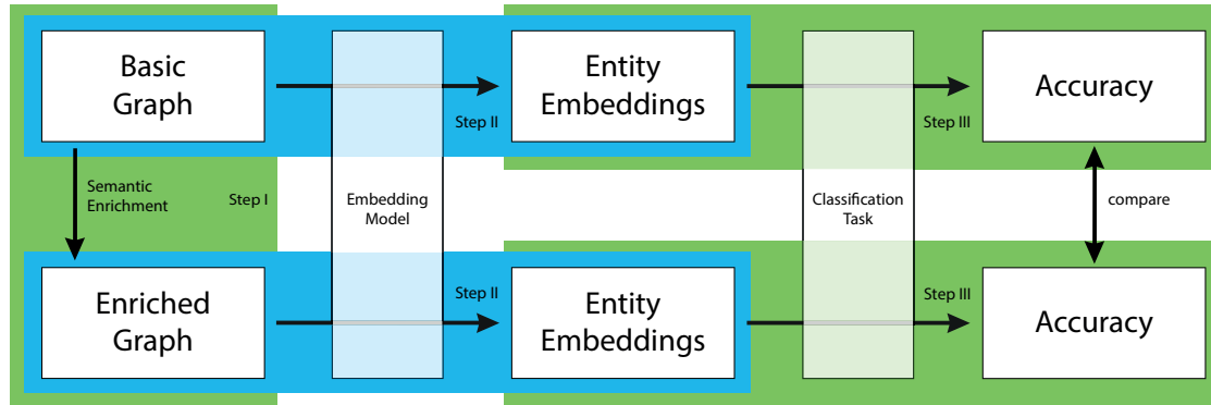
Figure 2: Experimental pipeline.
