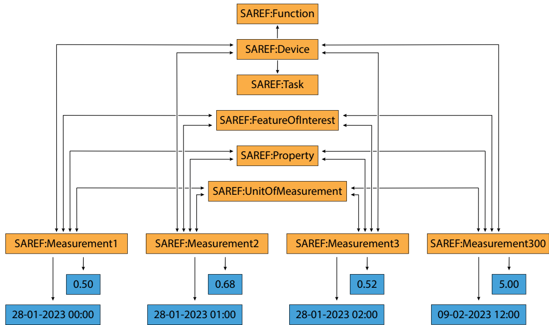
Figure 1: Subset of four measurements from a SAREF IoT graph, orange boxes are entities, blue boxes are literals. Arrow heads represent the direction of the properties.
